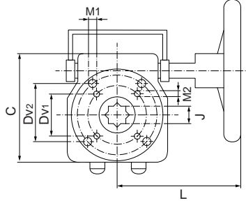
Quadro lato valvola / Valve Square
